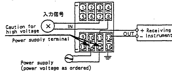
Fig.10 Wiring Diagram
